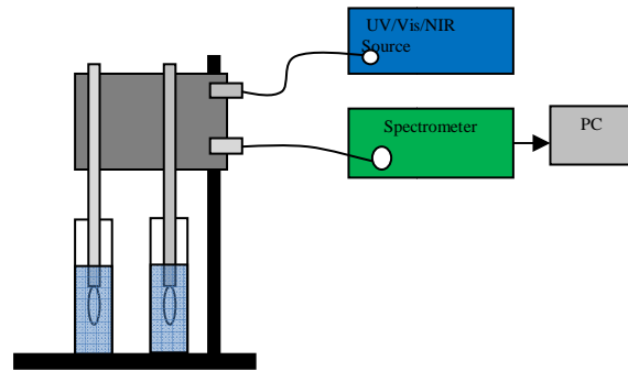
Figure 5. Experimental setup of CMEOF sensor array. A broadband source and a computer controlled spectrometer are used to interrogate the sensors.
